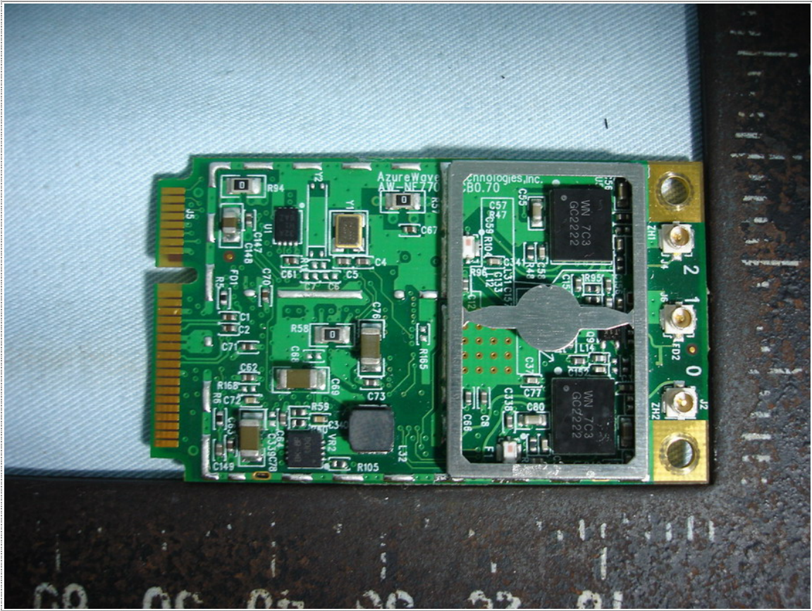
Front View of EUT-2 (AW-NE770)
