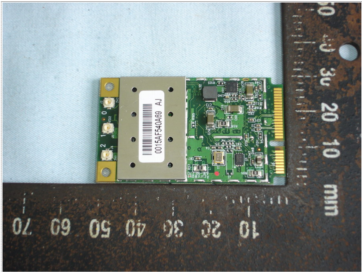
Front View of EUT-1 (AW-NE770)
