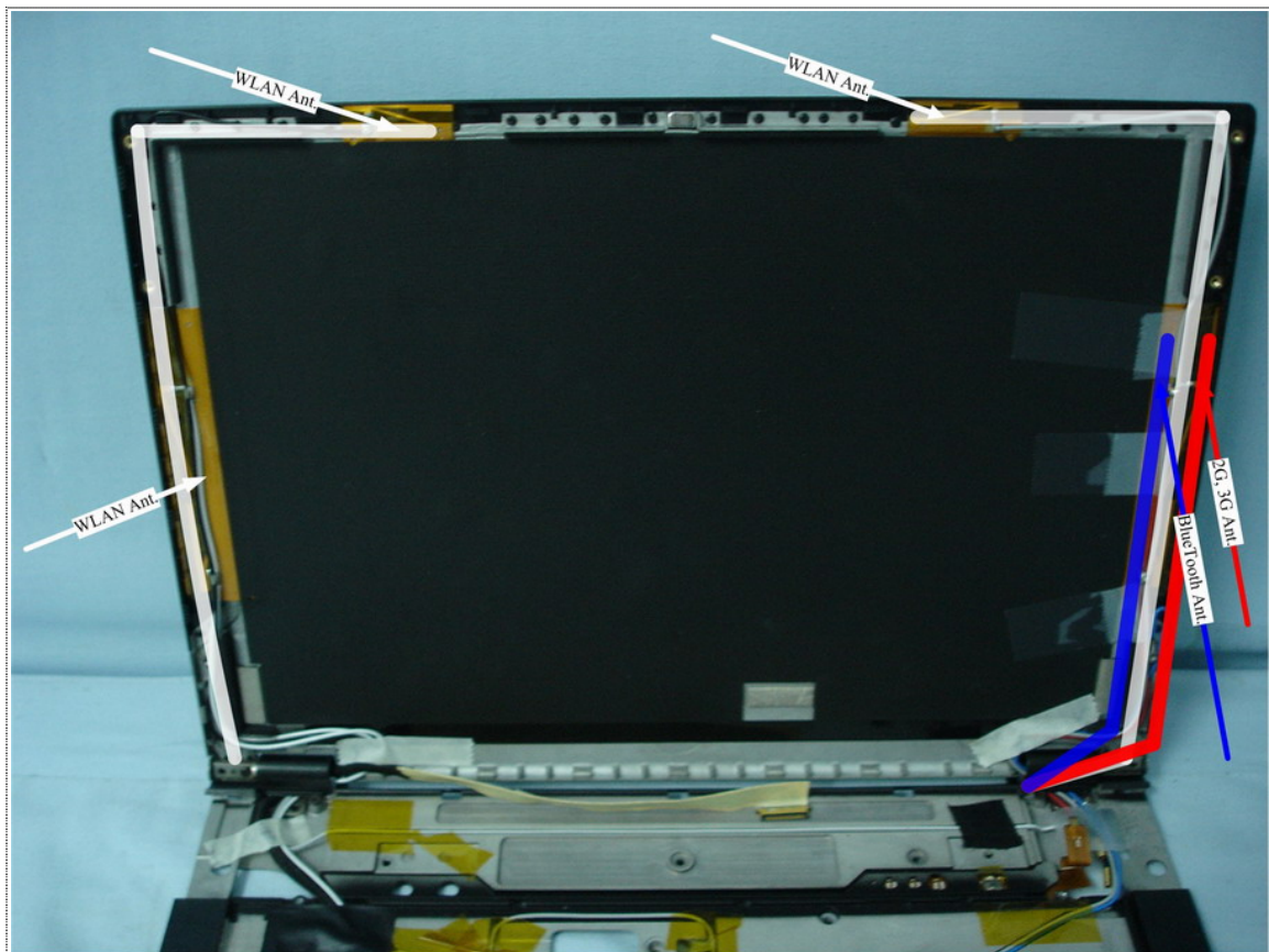
Antenna Location
