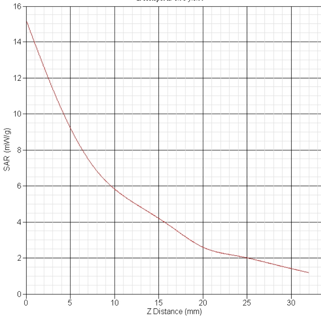
SAR-Z Axis at Hotspot x:-1.98 y:1.99
