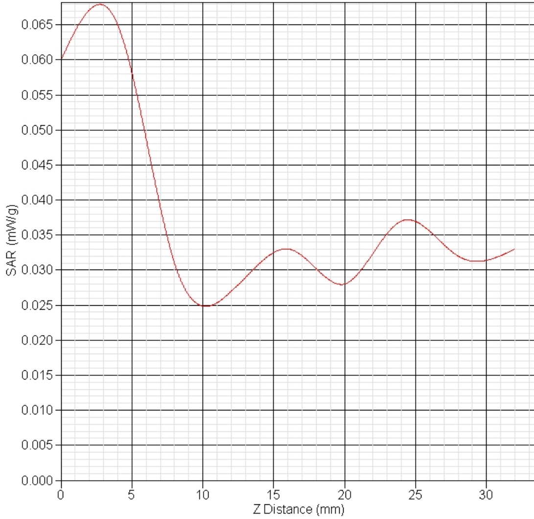
SAR-Z Axis at Hotspot x:-27.90 y:11.99
