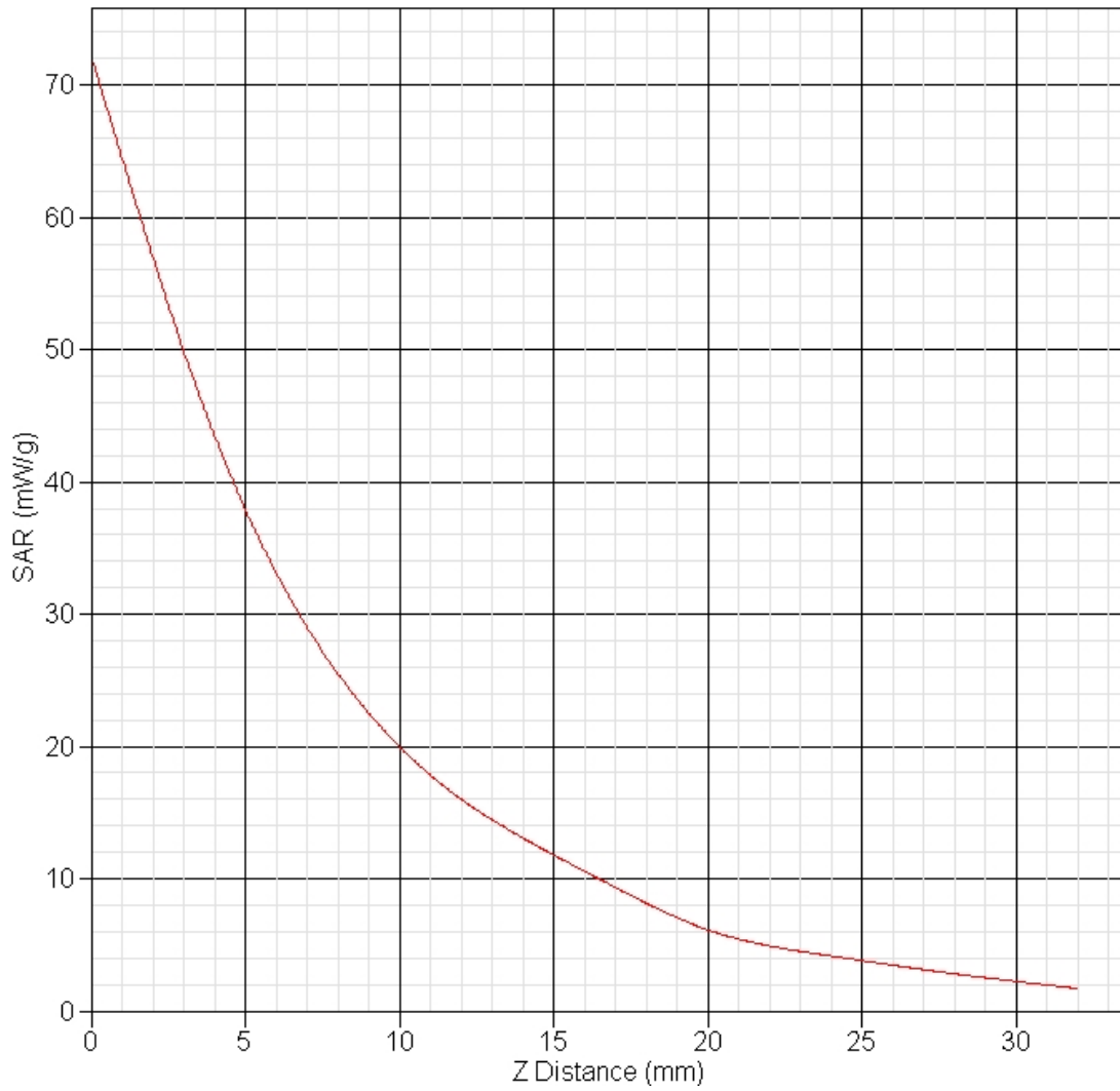
SAR-Z Axis at Hotspot x:0.08 y:-0.02
