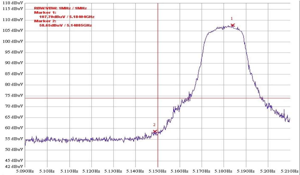
Dual Tx 802.11n (HT20) CH36 PK
