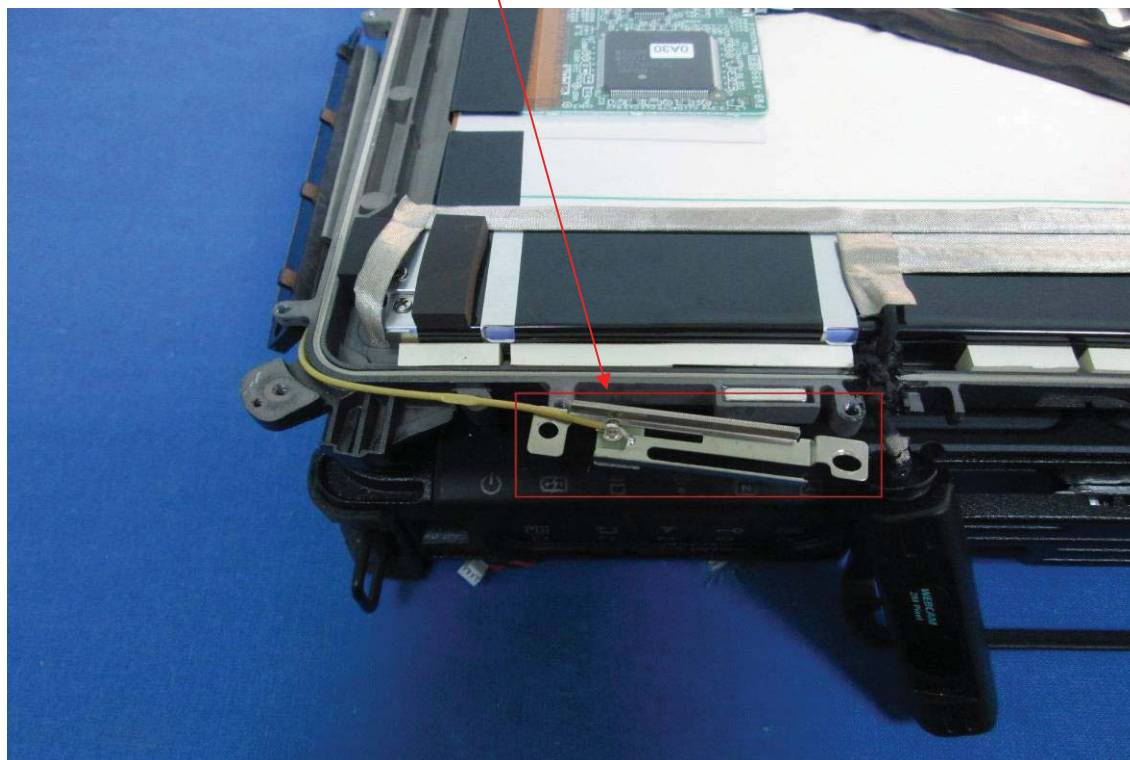
WLAN Antenna & BT Antenna
