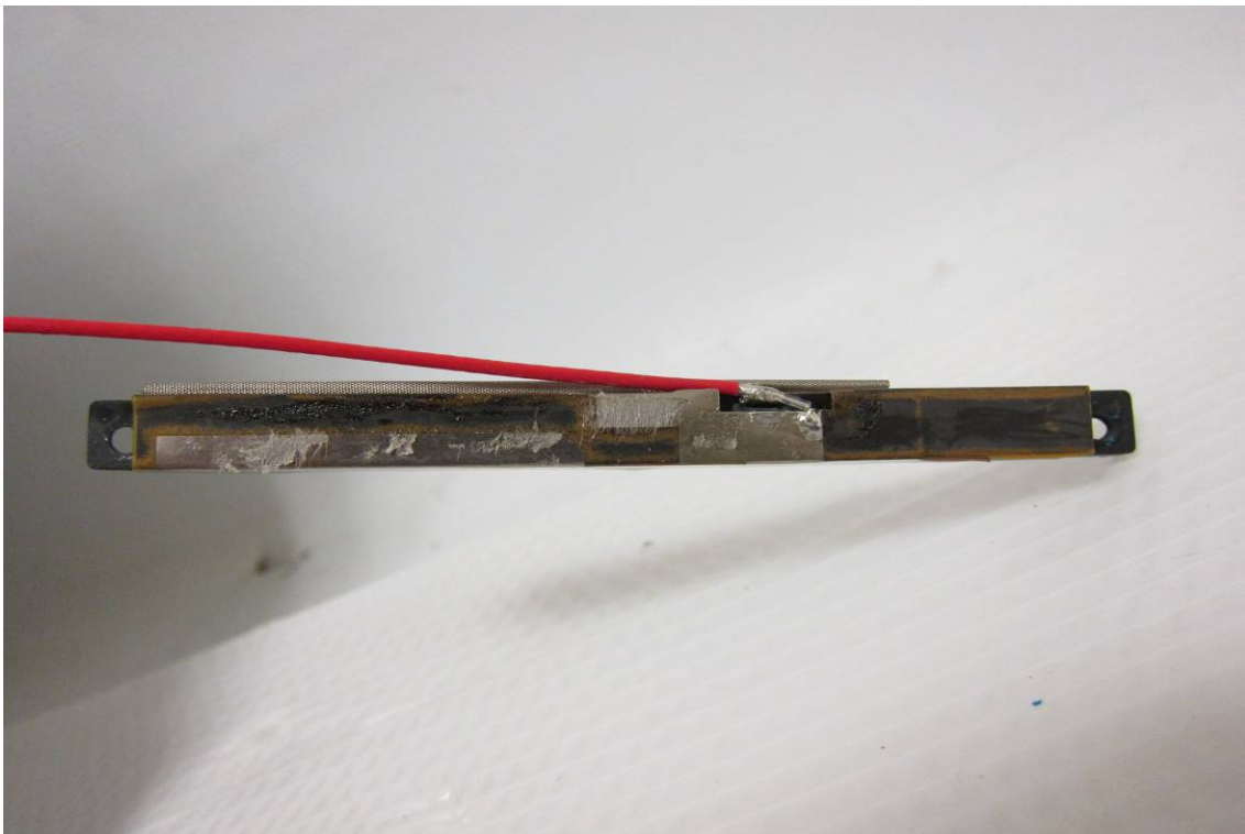
Internal View of WWAN Antenna (MAIN)
