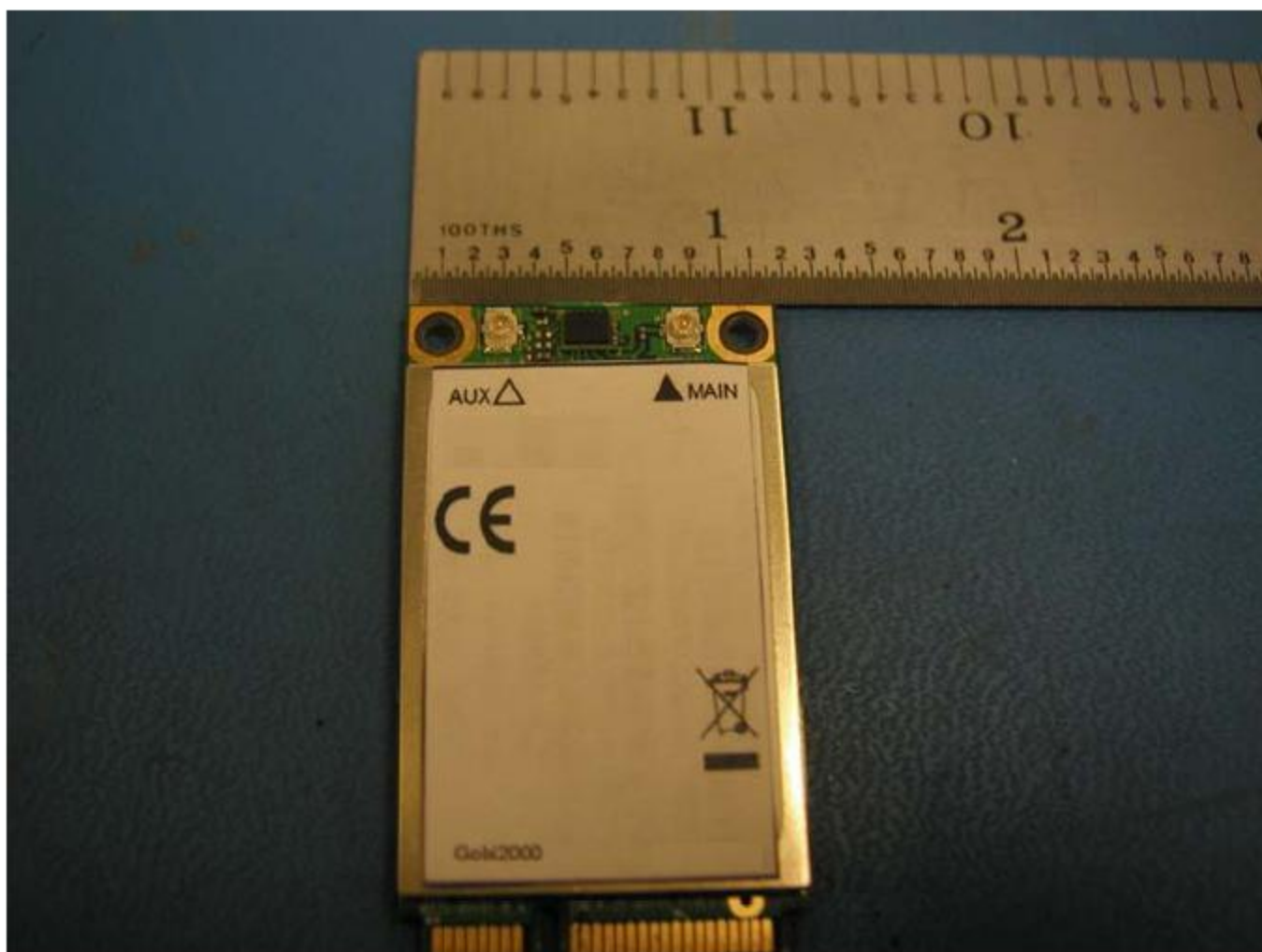
Figure 1 Gobi™2000 Module Rear External Photograph (Shields Removed)
