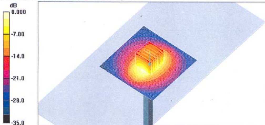
0 dB = 11.6mW/g
