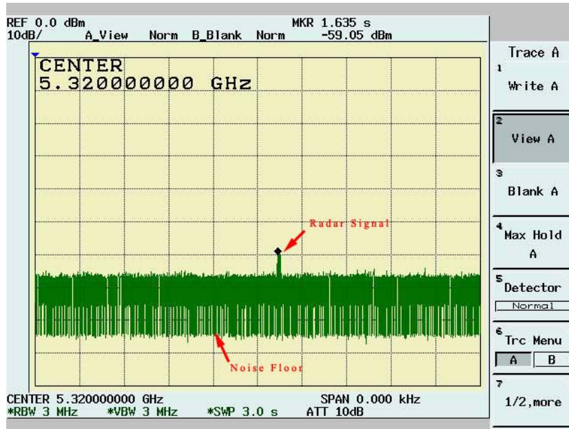
5320MHz Radar Signal 1(Step 2: Slave)
