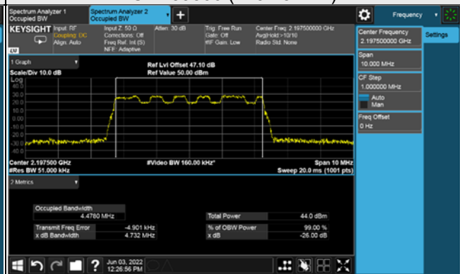
Ch 439500 (2197.5MHz)
