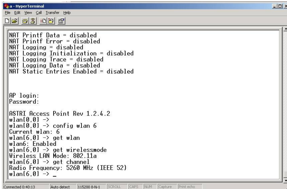
Figure 7. 802.11a in A8 BTS
