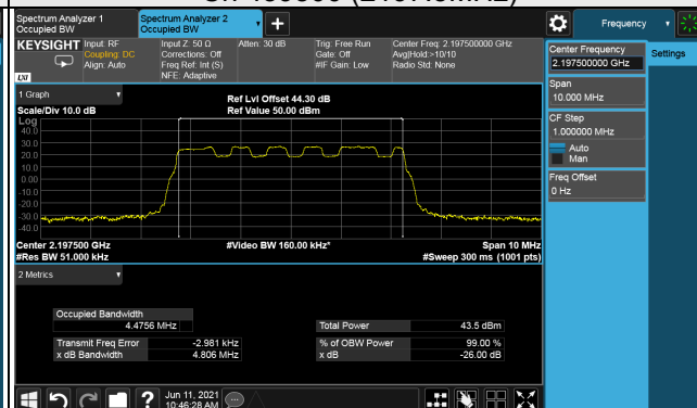
Ch 439500 (2197.5MHz)
