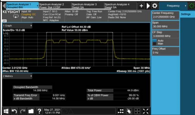
Ch 402500 (2012.5MHz)
