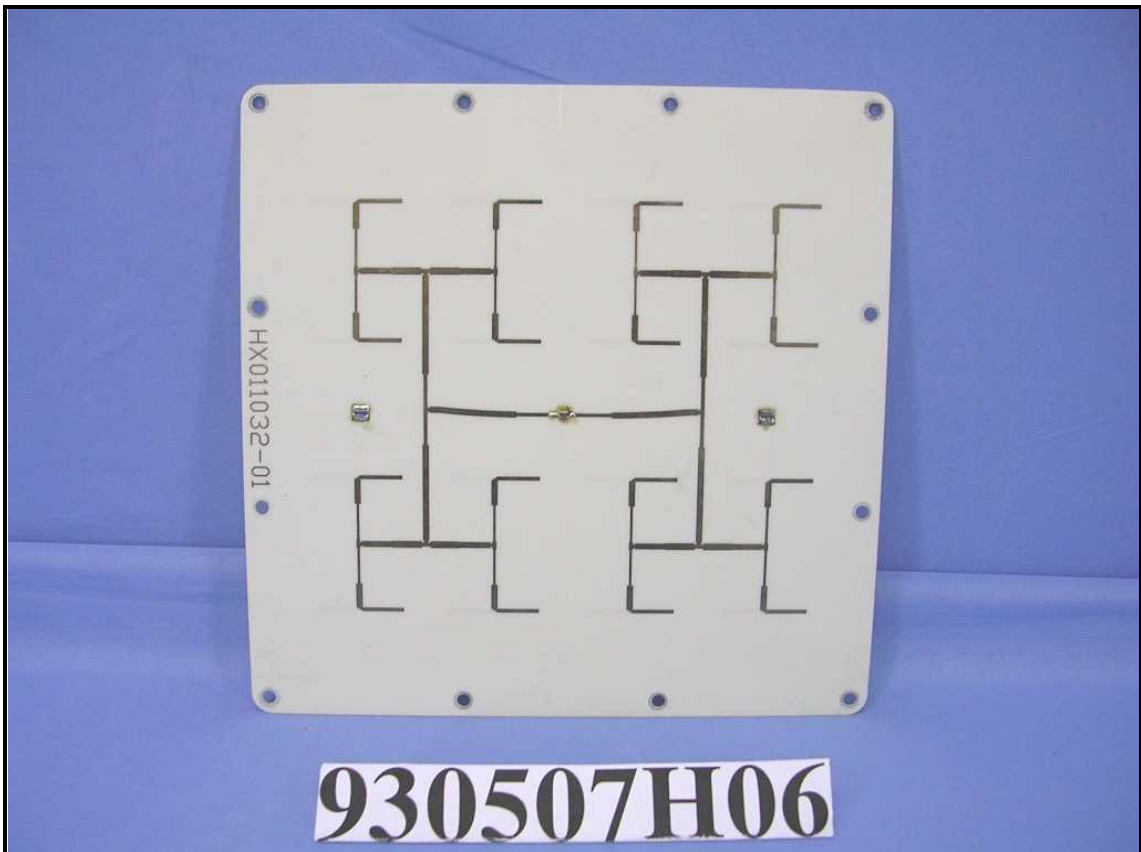
Antenna 1
