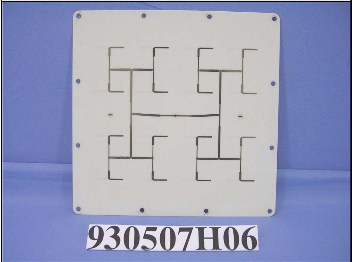
Antenna 1
