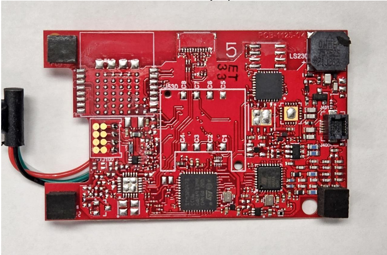
PCB Assembly-Top
