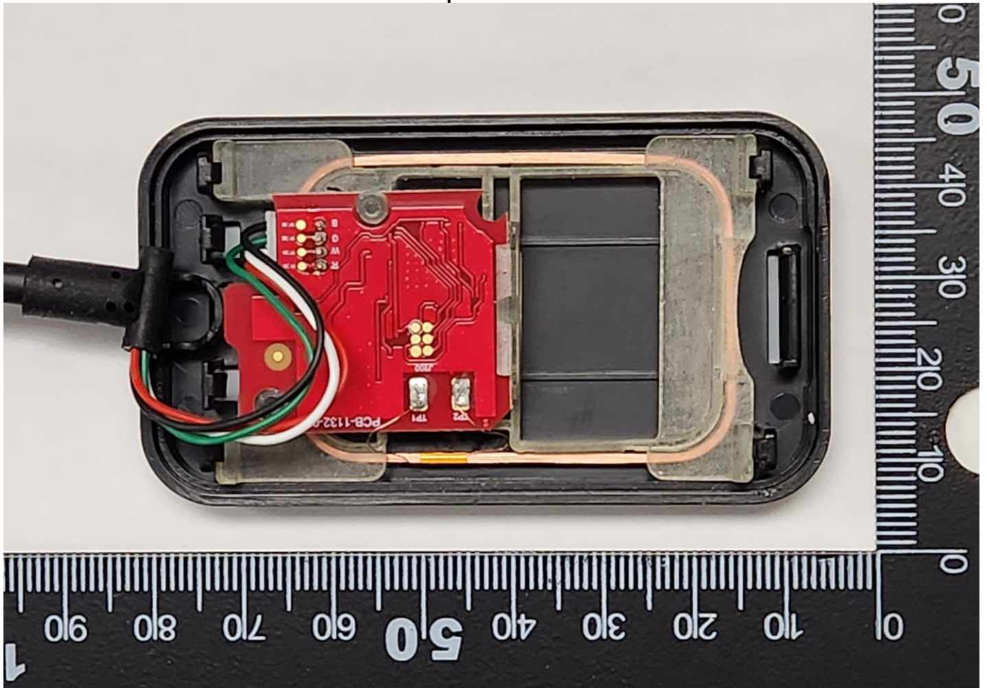
EUT Top cover removed
