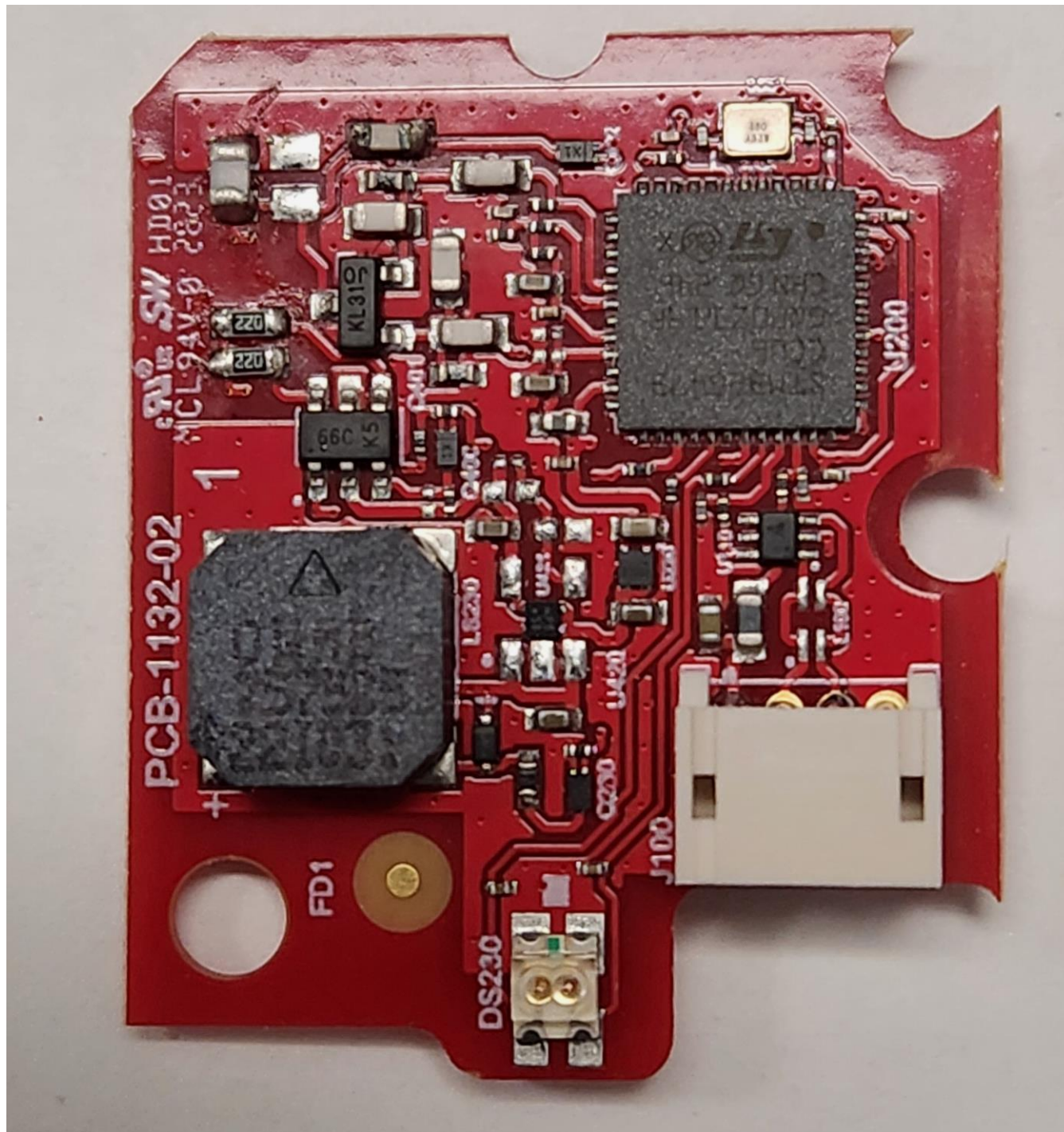
Top of Main PCB
