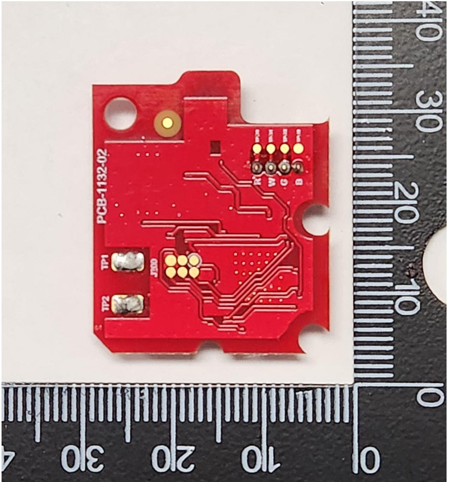
PC Board-Bottom
