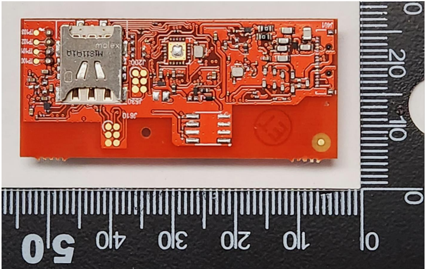
Main PC Board-Bottom
