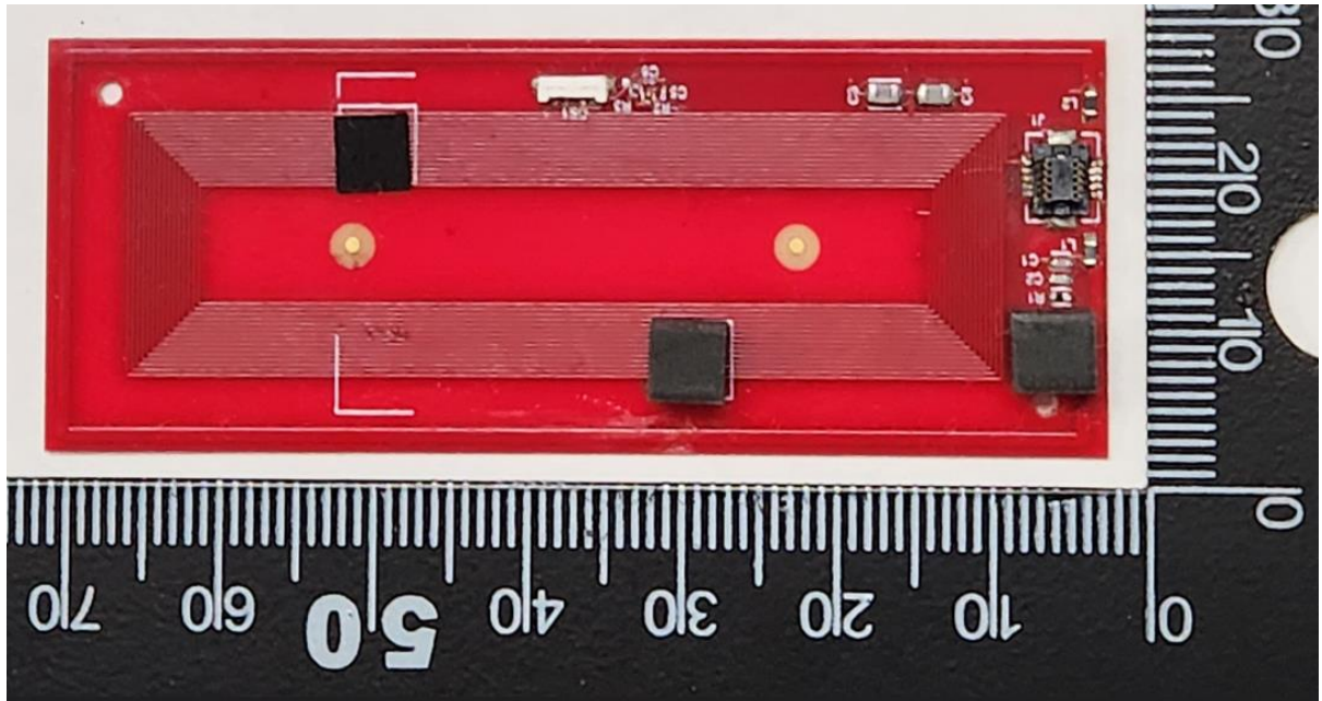
Antenna PCB top
