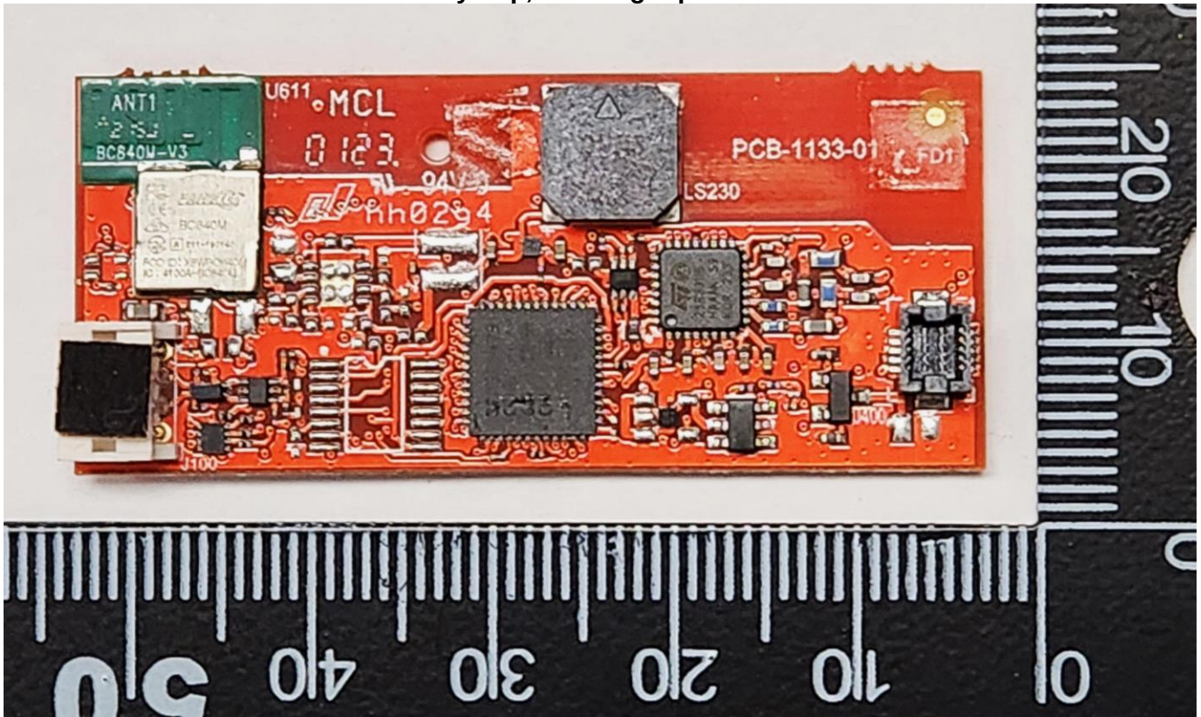
Assembly Top, showing top of Main PCB
