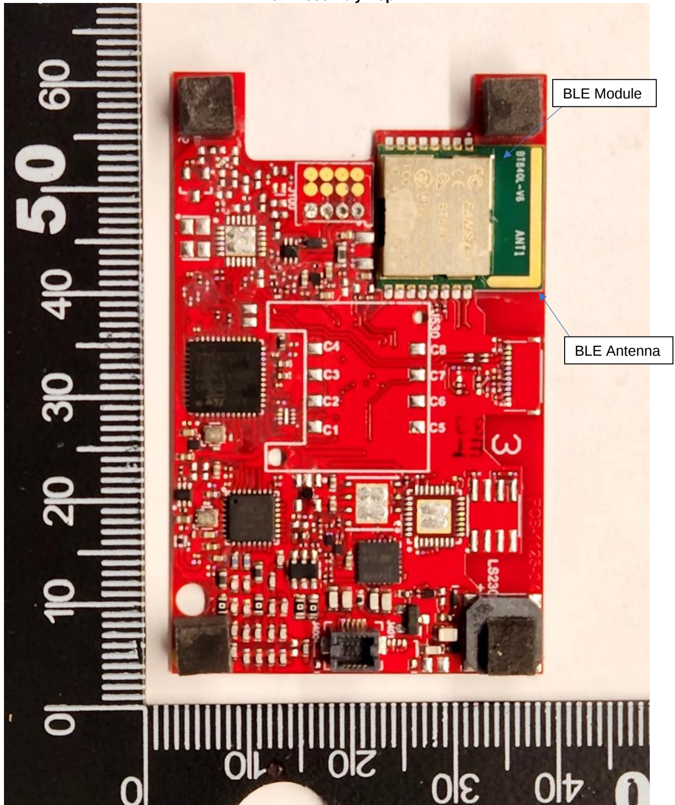
PCB Assembly-Top
