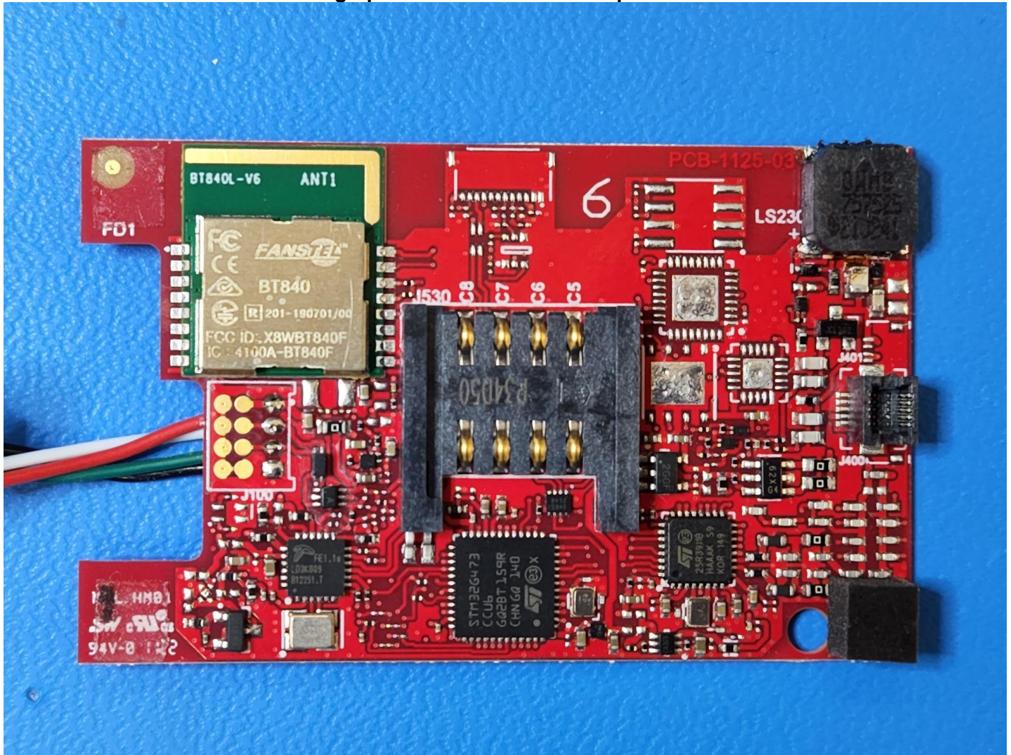
Photograph of 305 PC Board: Component Side
