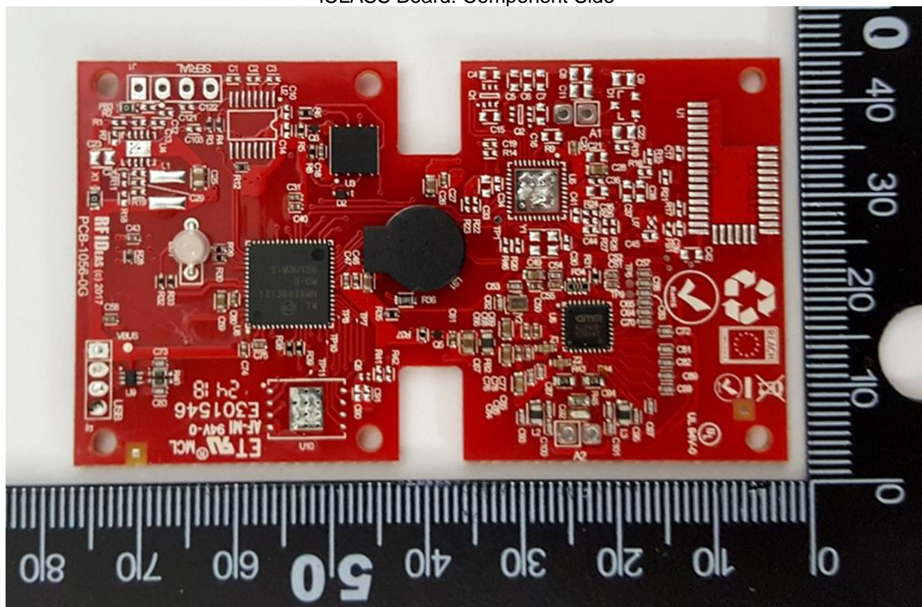
iCLASS Board: Component Side
