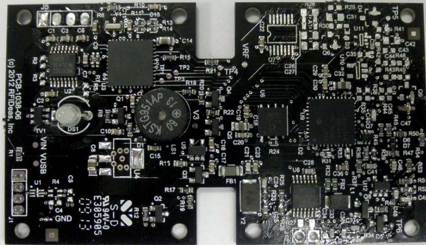
13.56MHz serial motherboard top view
