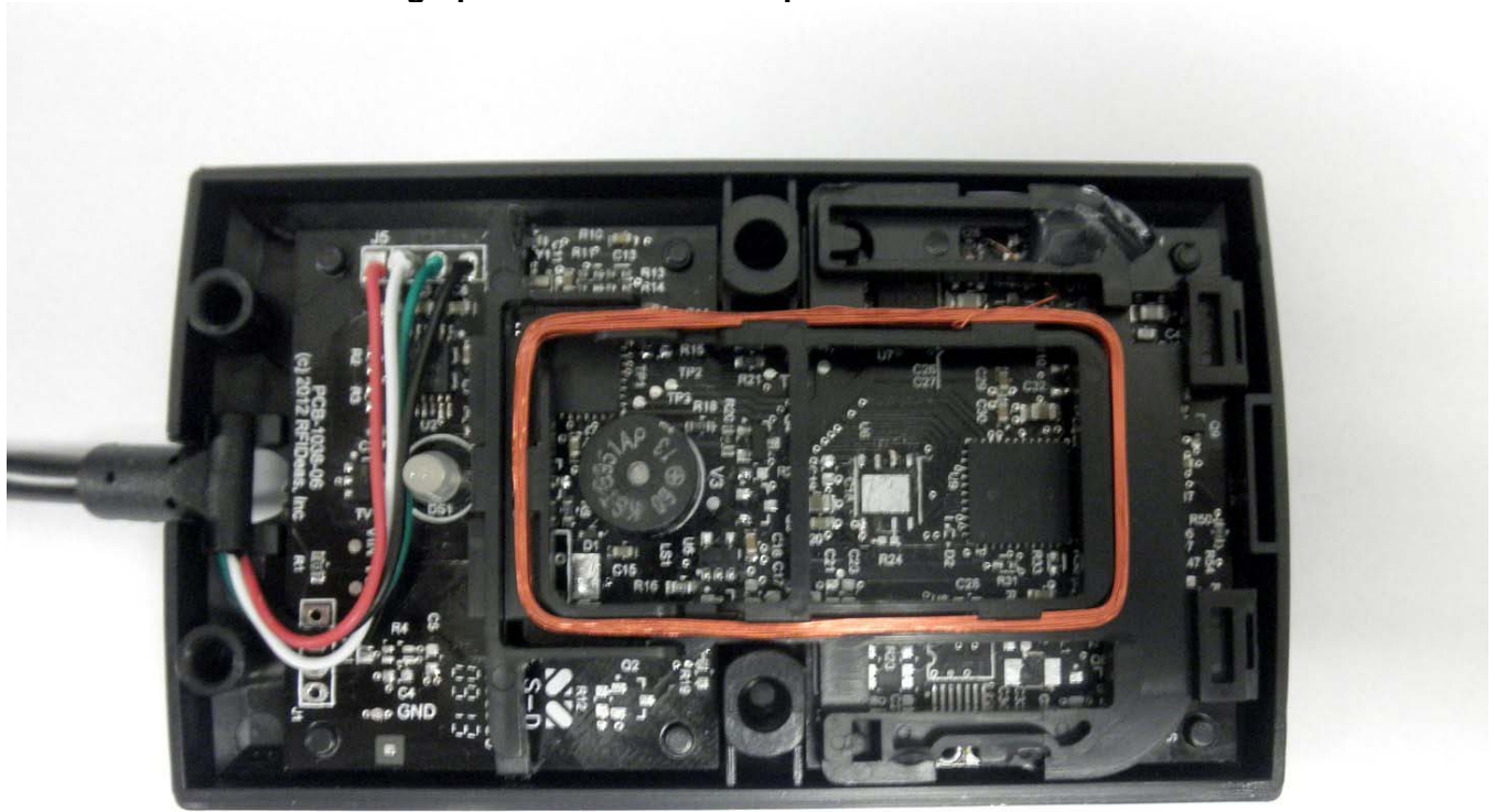
125KHz motherboard assembly top View
