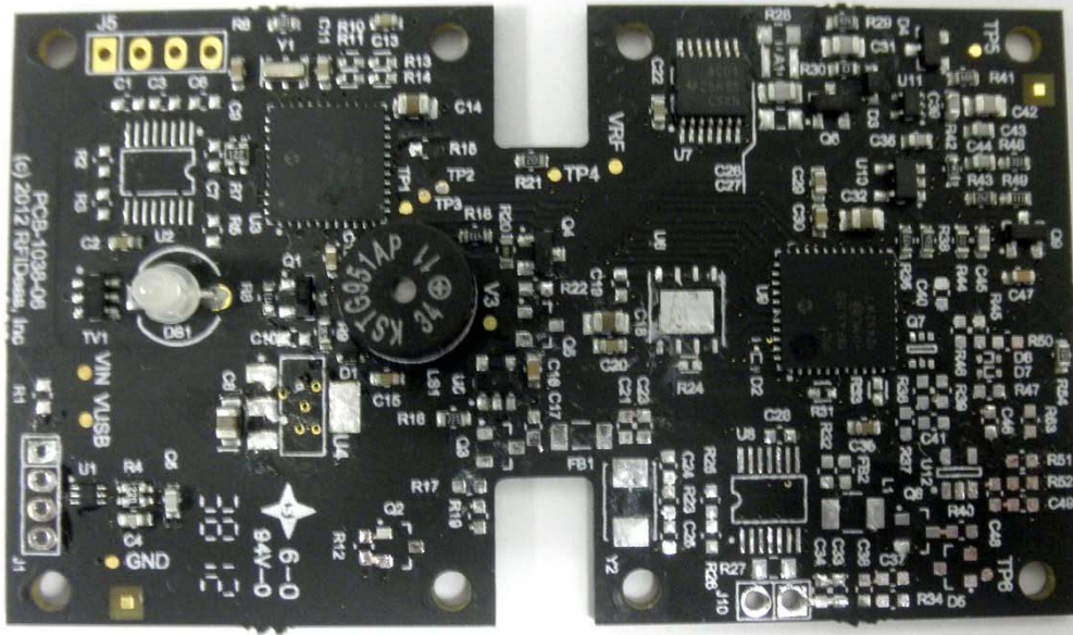
125KHz USB Motherboard Top View
