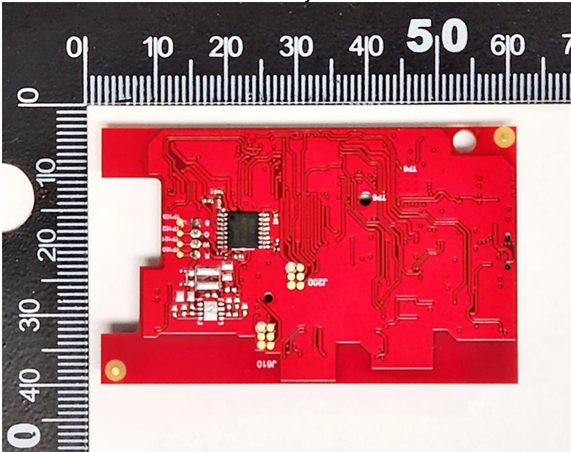
PCB Assembly-Bottom
