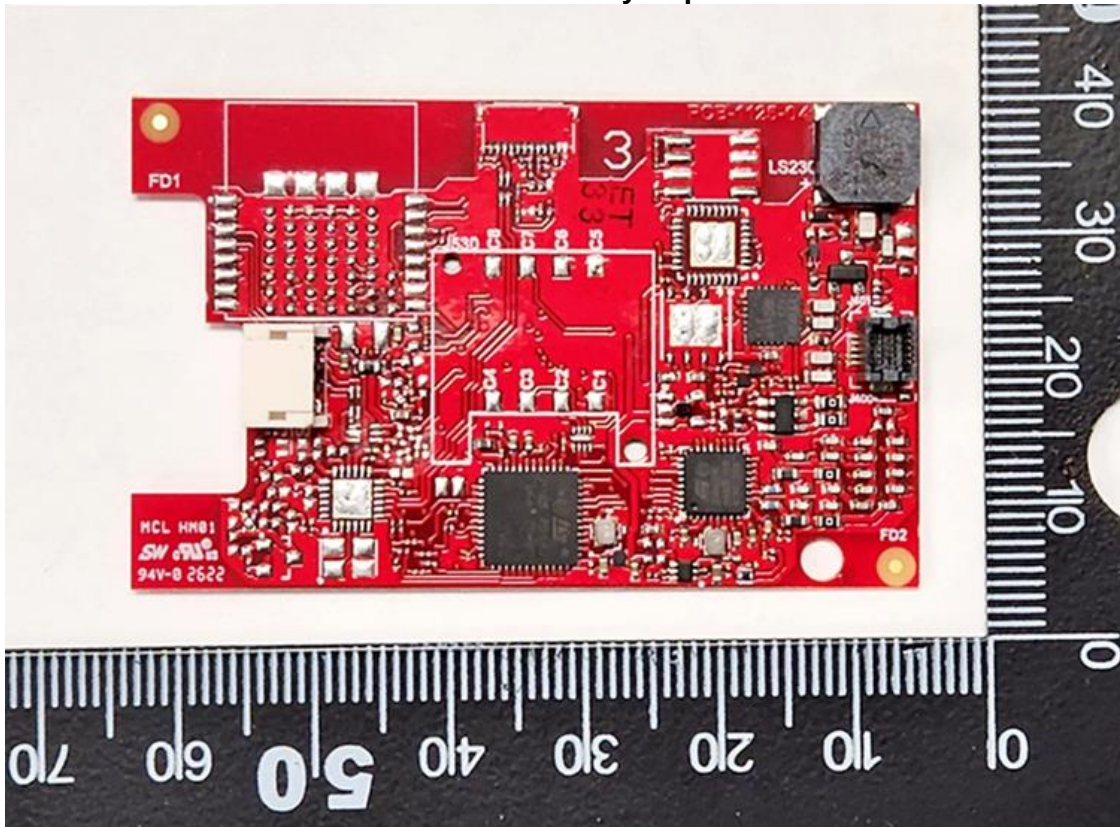
PCB Assembly-Bottom
