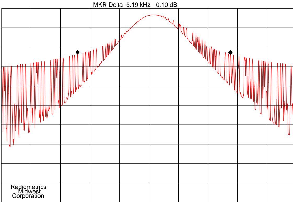
Figure 4. Occupied Bandwidth Plot 13.56 MHz
