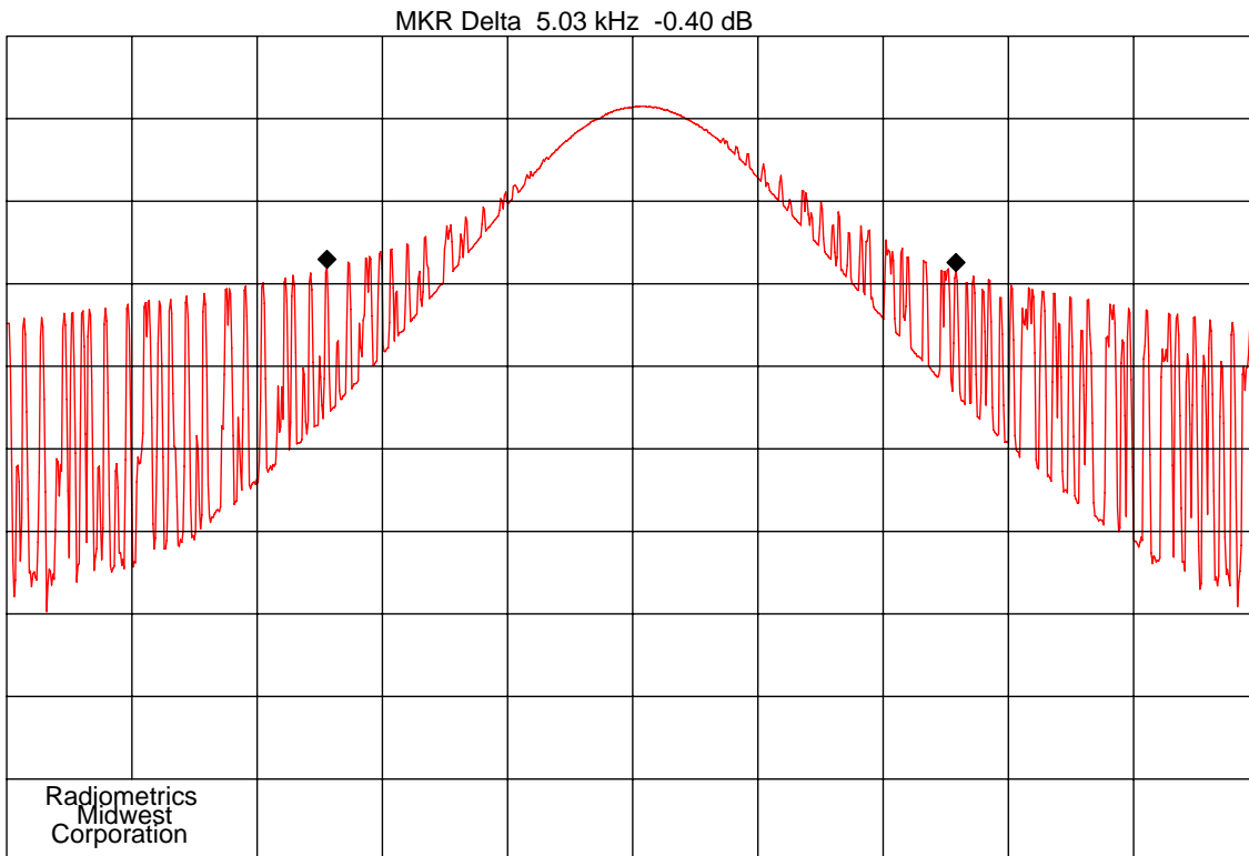
Figure 3. Occupied Bandwidth Plot 125 kHz
