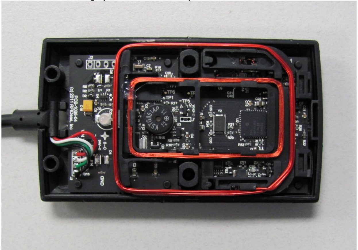
Photograph of PC Board: Component Side with Antenna
