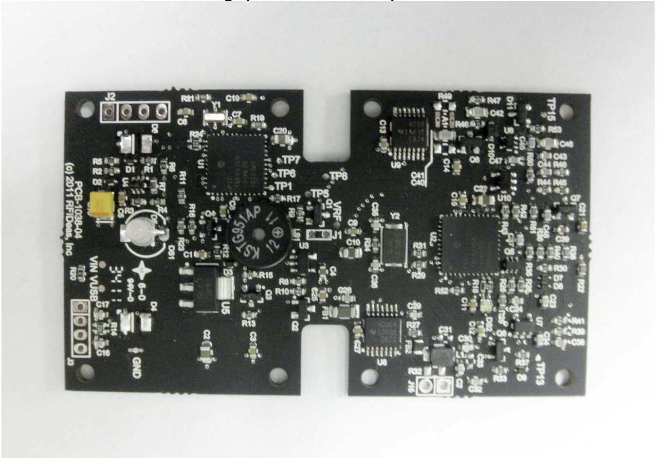
Photograph of PC Board: Component Side
