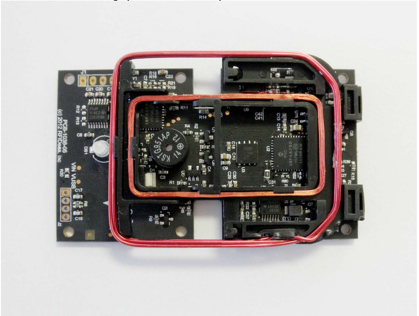
Photograph of PC Board: Component Side with Antenna
