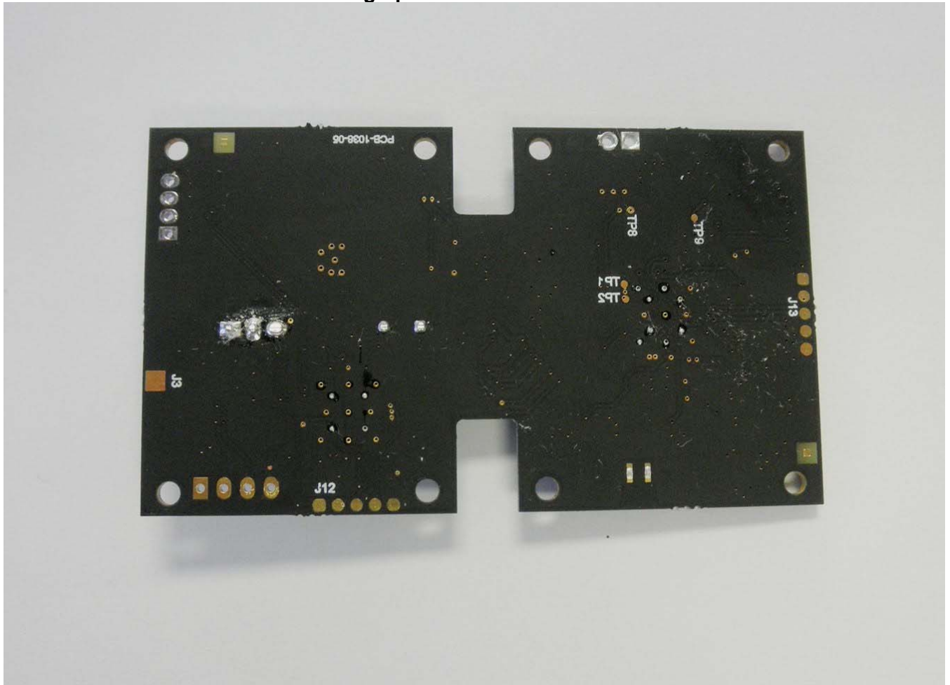
Photograph of PC Board: Foil Side
