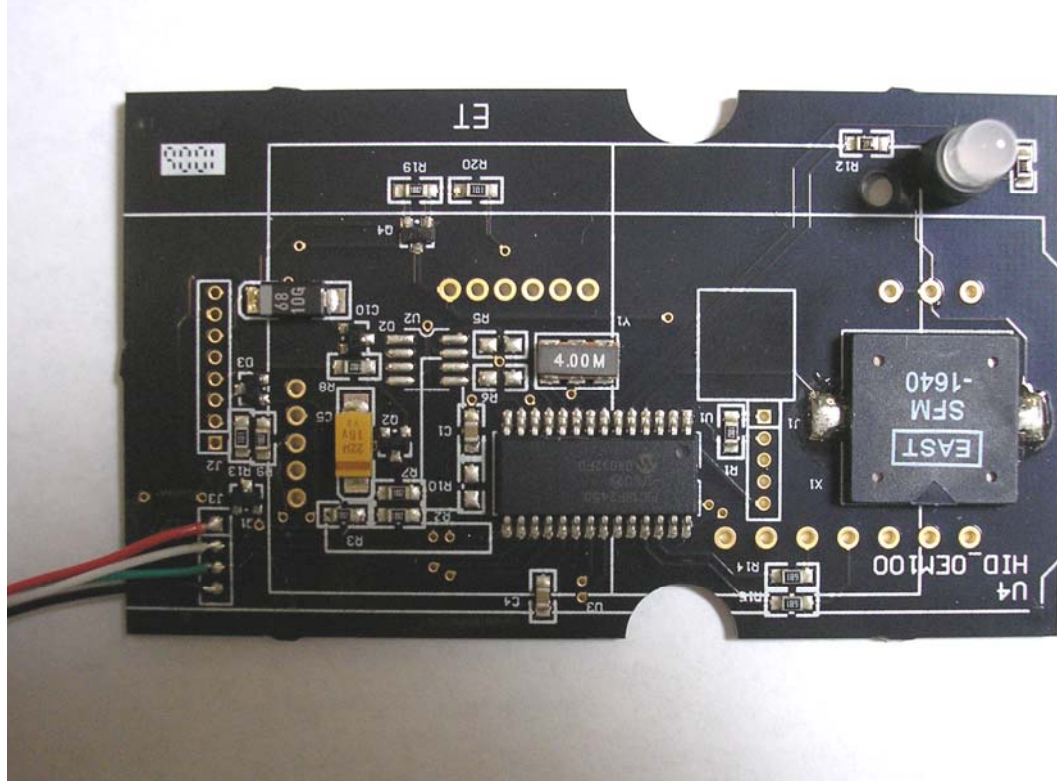
Photograph of Component Side of Controller PCB
