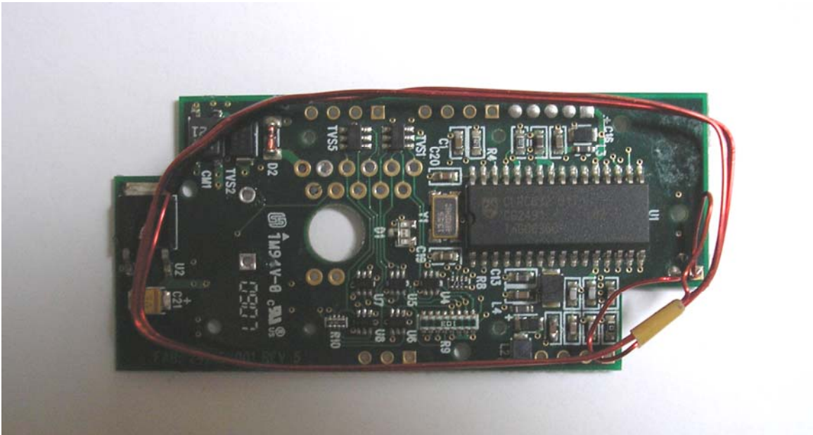
Photograph of Component side of RF PCB showing Antenna
