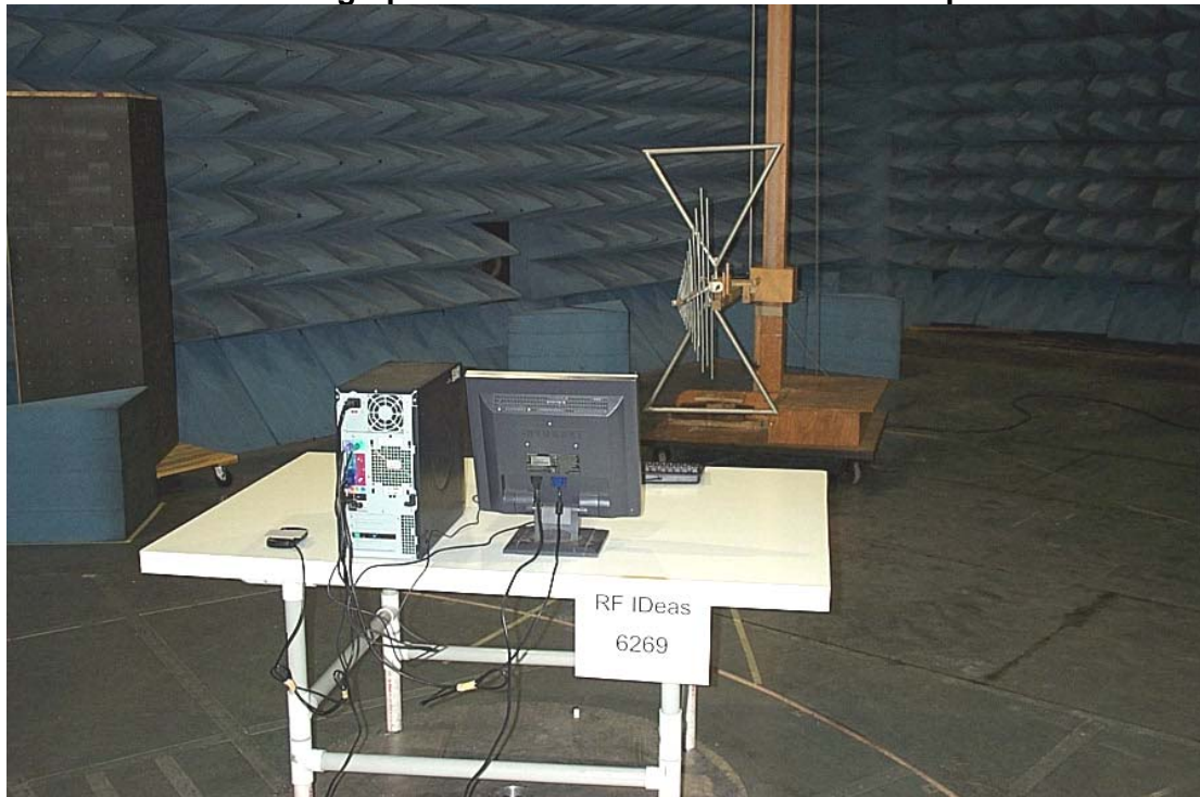
Electric Field (above 30 MHz)
