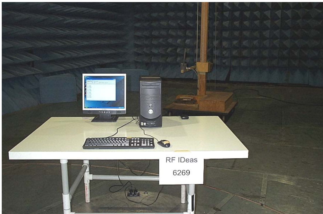
Magnetic Field (below 30 MHz)
