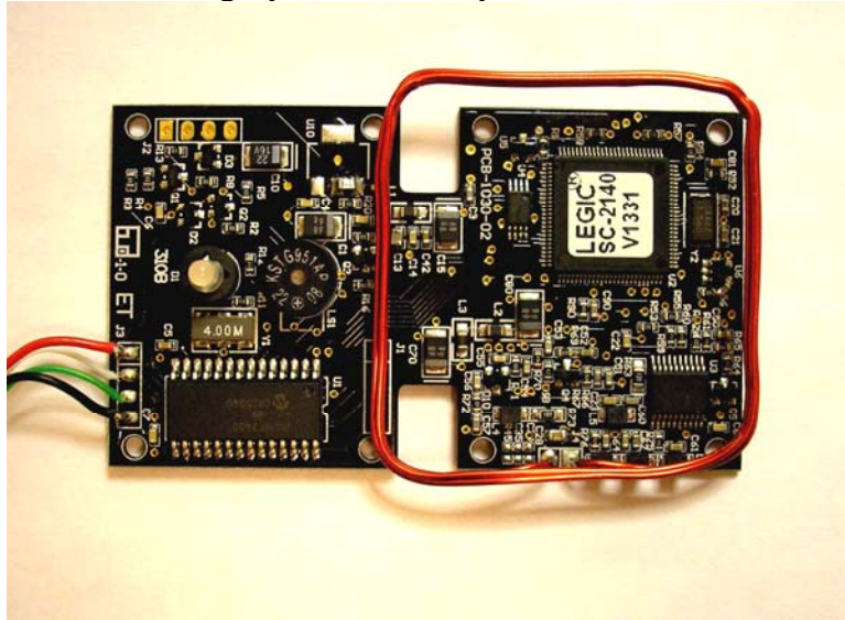
Photograph of front of processor board
