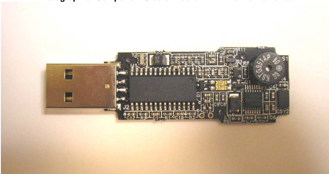
Photograph of Component Side of Board with Antenna Removed
