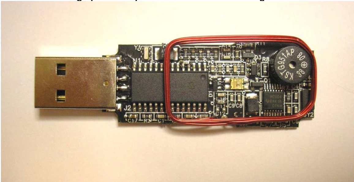
Photograph of Component Side of Board showing Antenna
