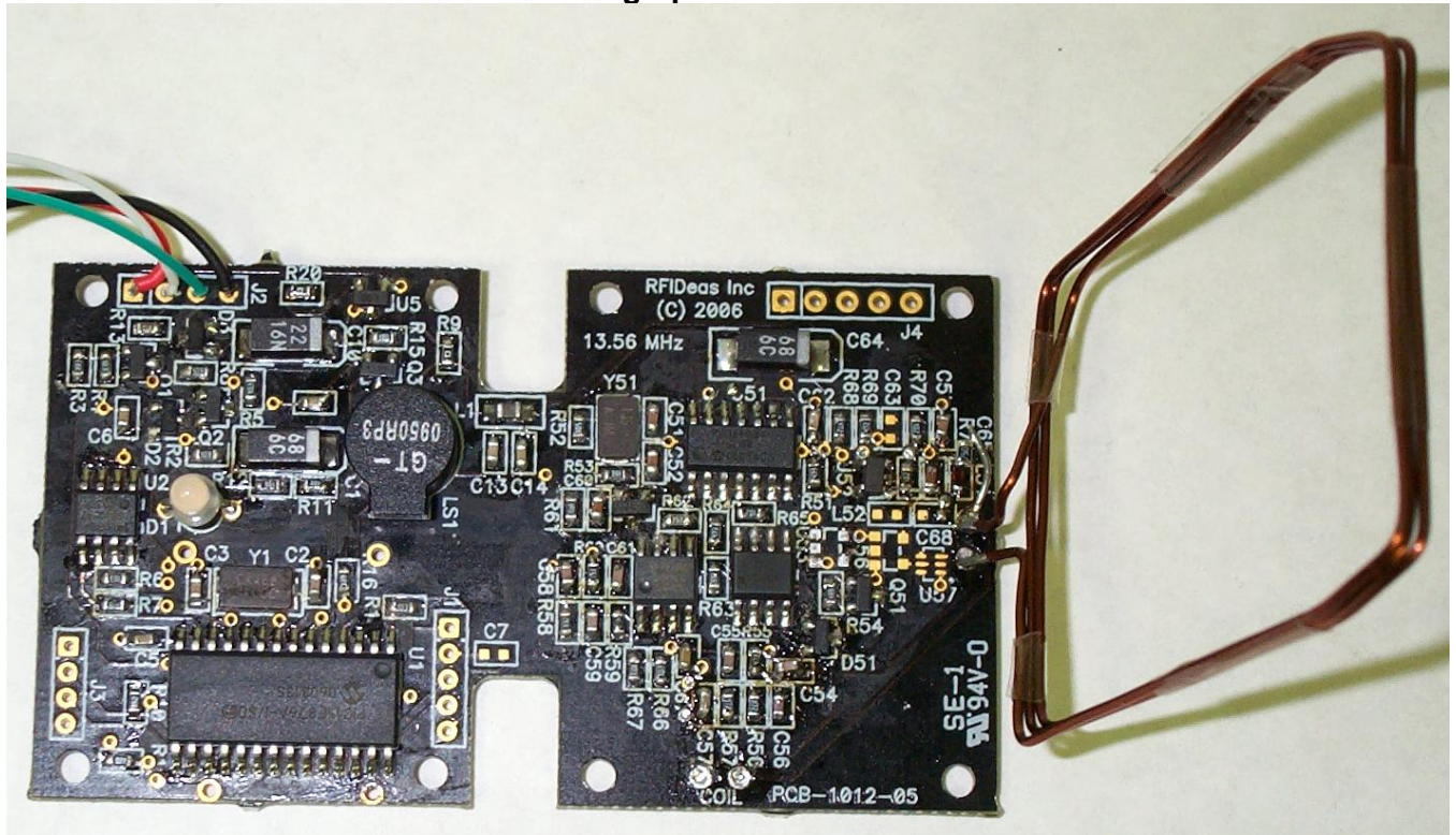
Photograph of PCB: Front
