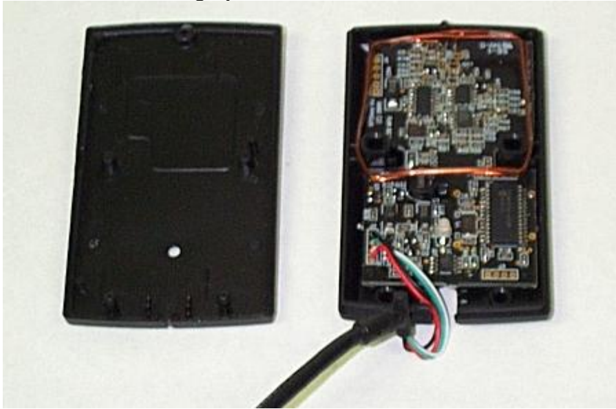
Photograph of EUT: Cover Removed
