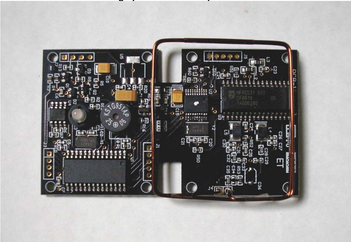
Photograph of Board: Component Side
