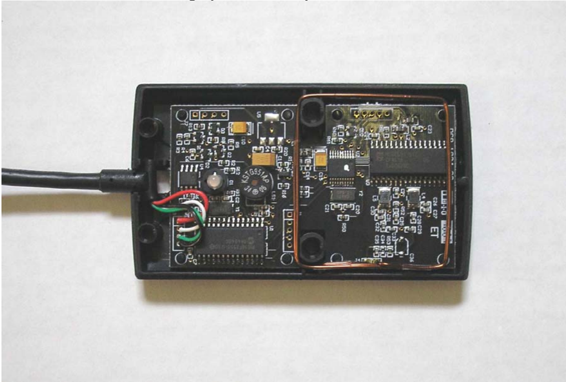
Photograph of EUT: Top cover removed
