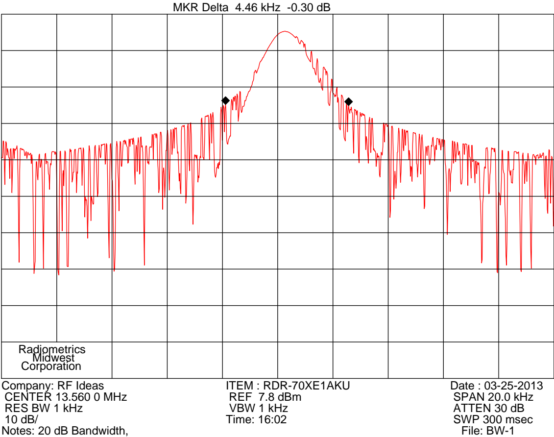
Figure 3. Occupied Bandwidth Plots 13.56 MHz
