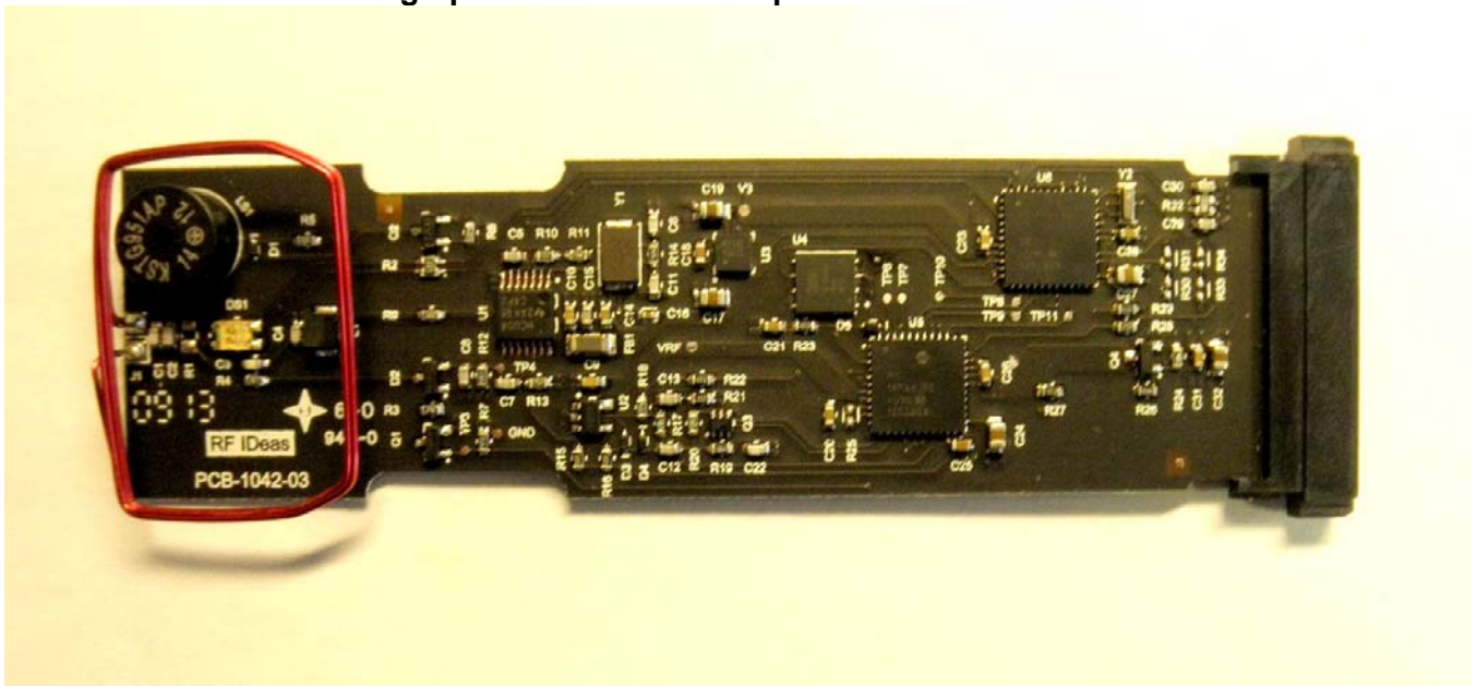
Photograph of PC Board: Component Side with Antenna
