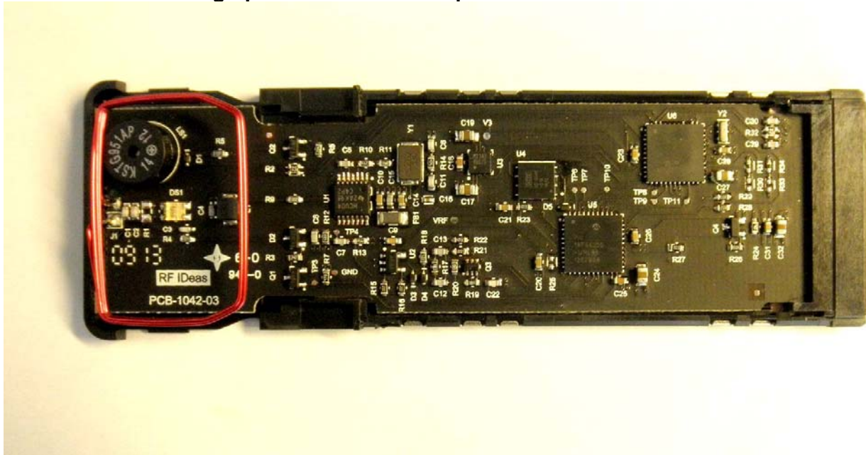
Photograph of PC Board: Component Side with Antenna
