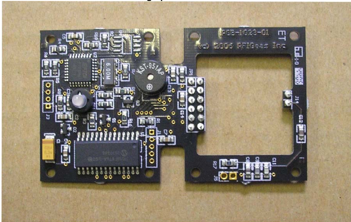
Photograph of PCB: Front
