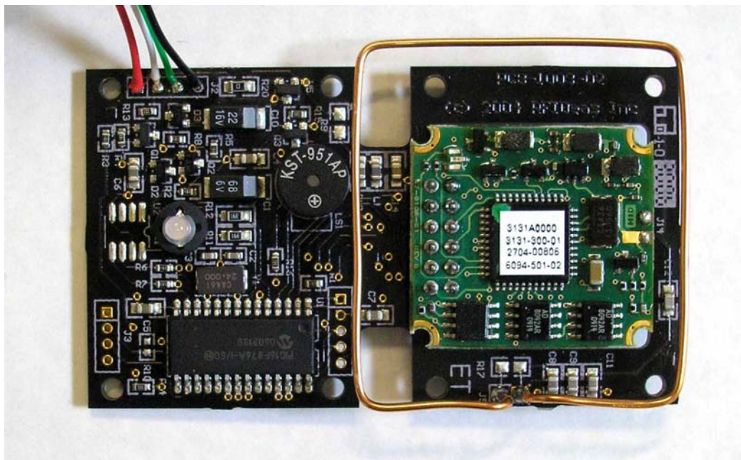
Photograph of Component side of RF PCB showing Antenna
