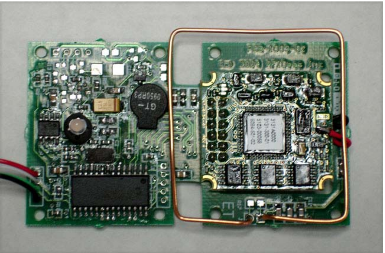
EUT PCBs Assembled
