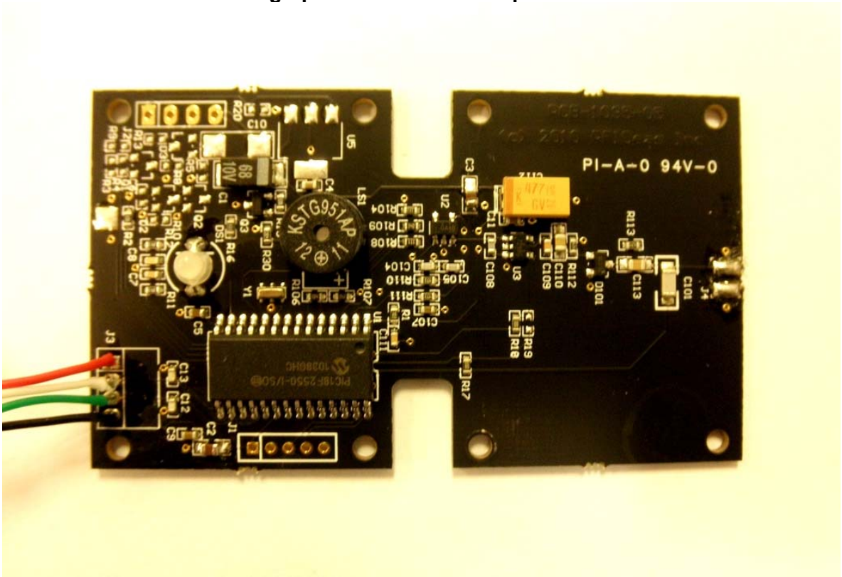
Photograph of PC Board: Component Side
