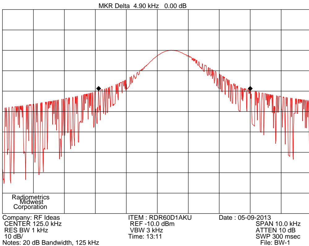
Figure 3. Occupied Bandwidth Plot
