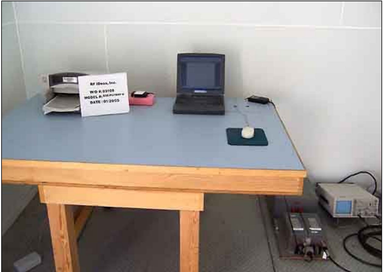
Mains Conducted Emissions - Front View - USB
