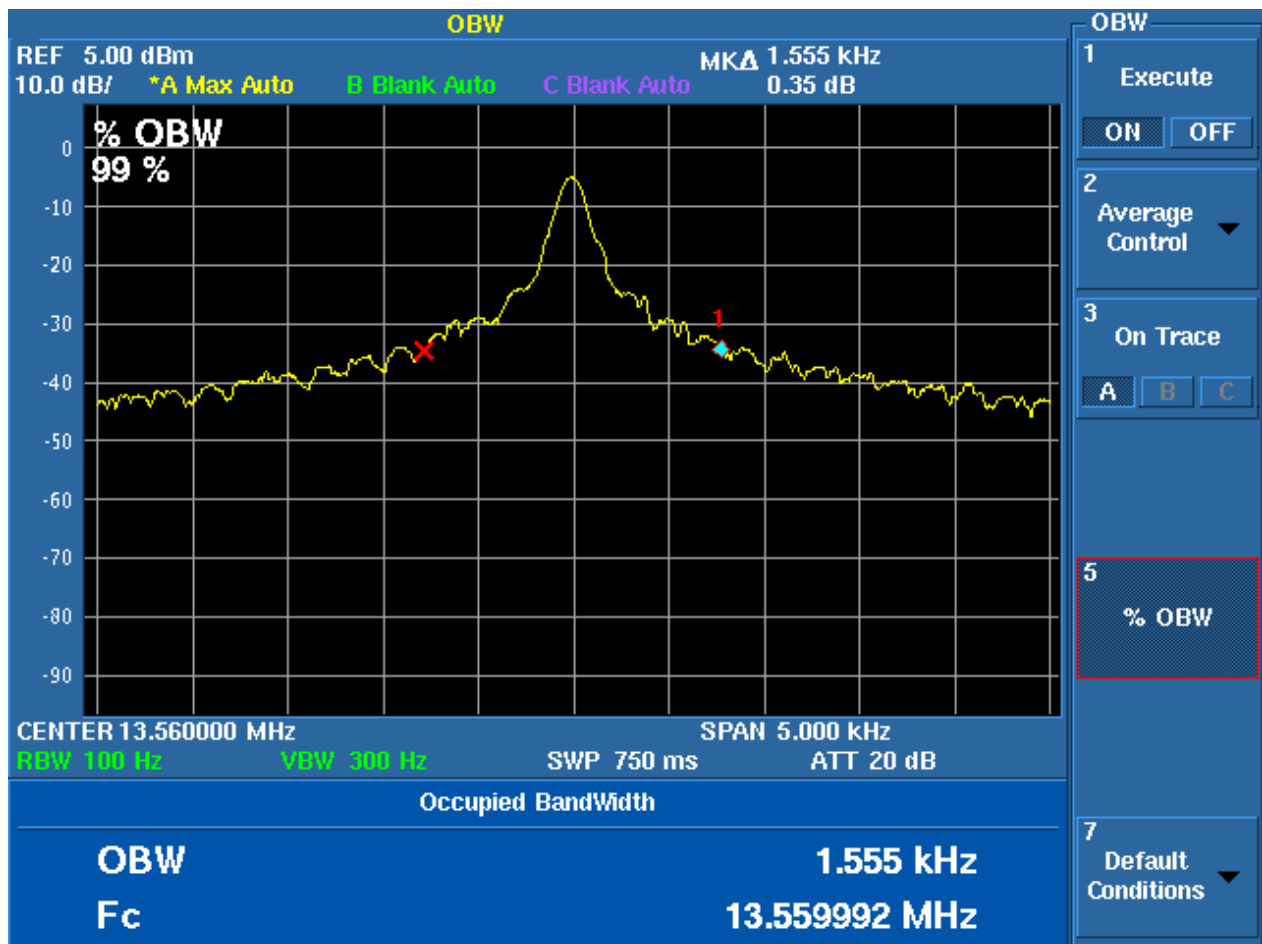
Figure 3. Occupied Bandwidth Plot
