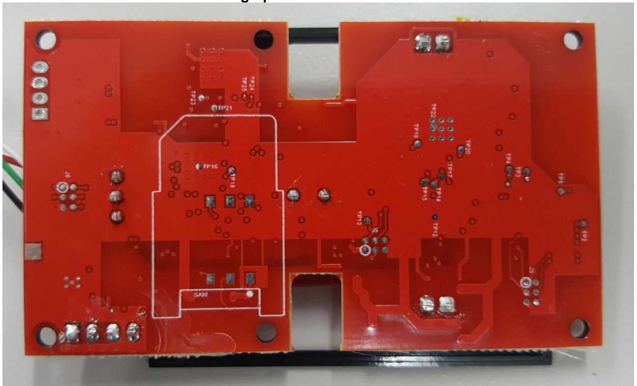
Bottom of PCB for all boards
