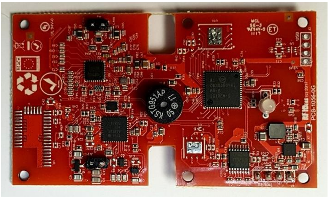
Photograph of PC Board: Foil Side
