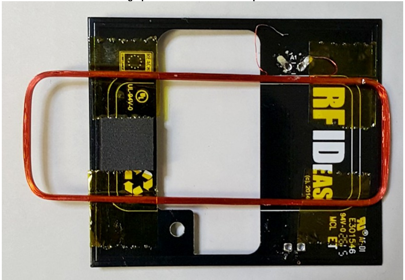
Photograph of Antenna Board: Component side
