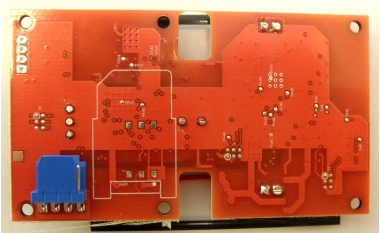
Photograph of PC Board: Foil Side
