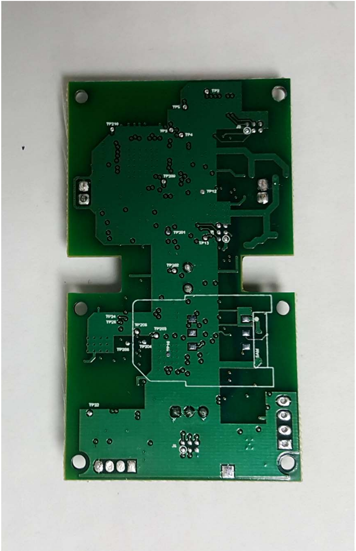
Photograph of PC Board: Foil Side
