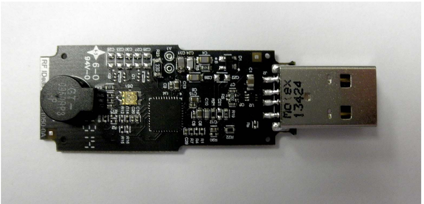
Component Side: Antenna removed
