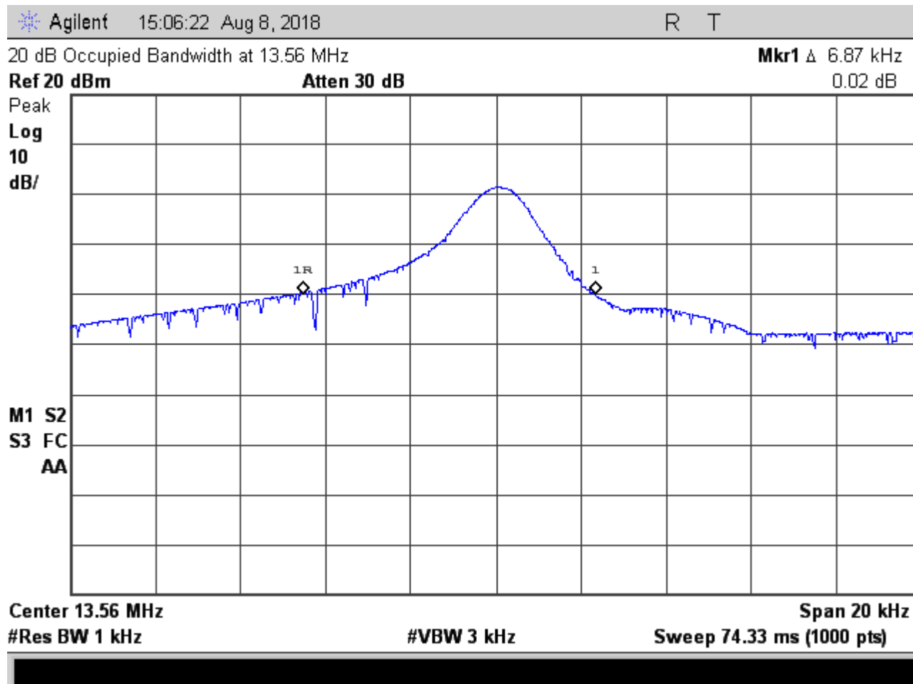
Figure 4. Occupied Bandwidth Plots 13.56 MHz
