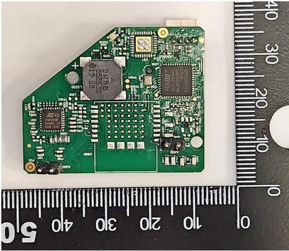
PC Board-Bottom
