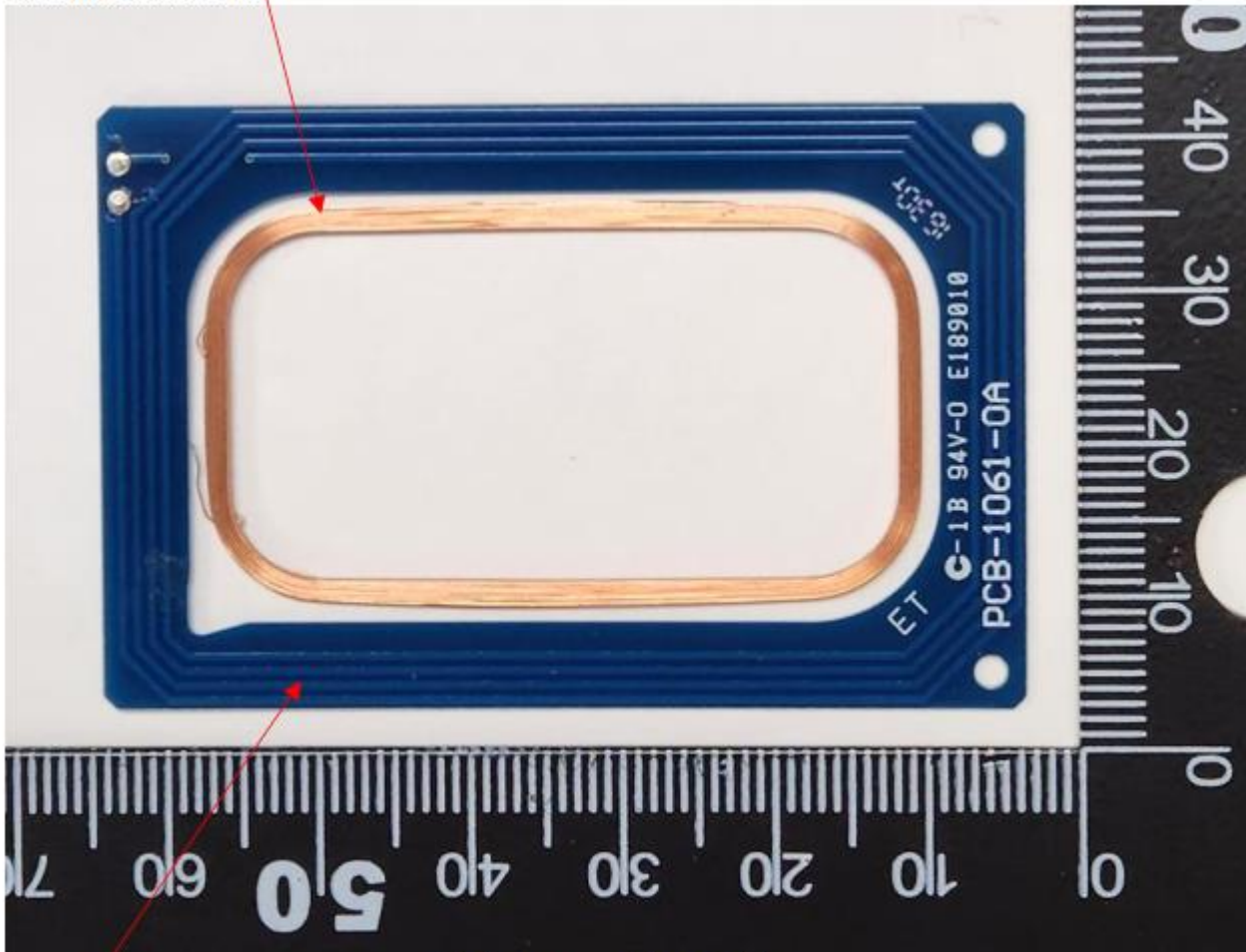
Antenna - Top Side
