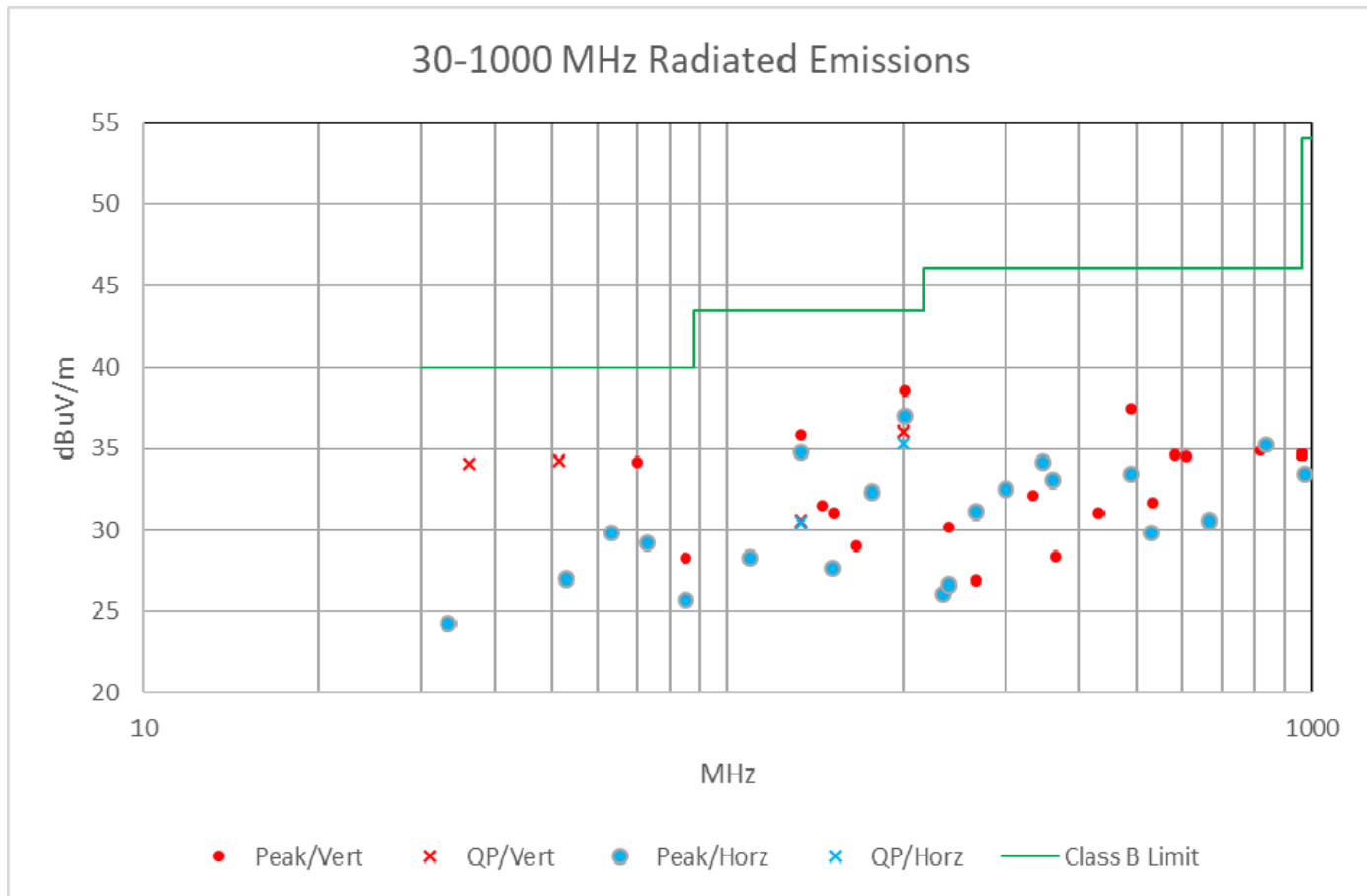
Radiated emissions in a graphical format. The above chart is the same data as the previous table.
